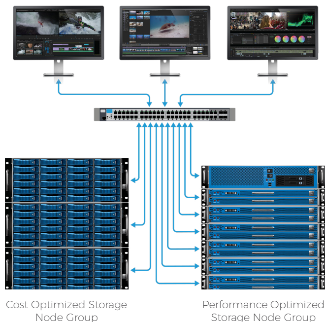
EFS storage cluster with performance-optimized and cost-optimized storage node groups
